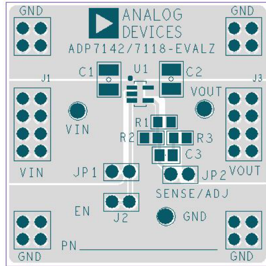
Figure 66. Example TSOT PCB Layout
