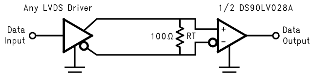
Figure 4. Point-to-Point Application
