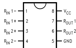
Figure 1. SOIC See Package Number D(R-PDSO-G8)
