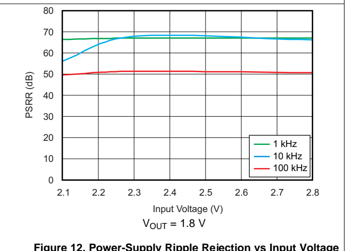
Figure 12. Power-Supply Ripple Rejection vs Input Voltage
